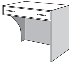
f Right Facing Open with convertible drawer cutout on left L02A
